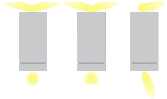
Lambertian
