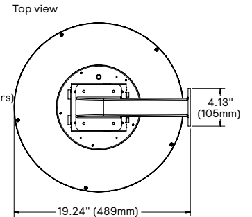
Wall mount
