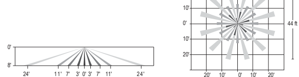
IMRI3 Luminaire or remote mount controller with #3 lens
