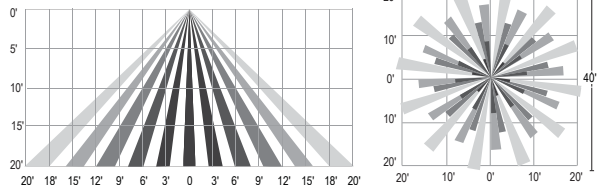
IMRI3 Luminaire or remote mount controller with #3 lens
